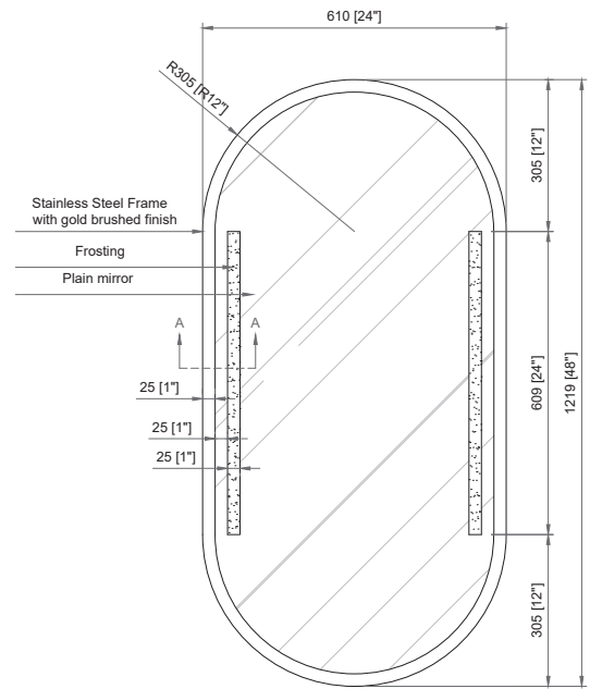
Front view Scale 1:8
