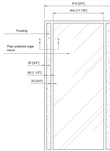
Front view Scale 1:8
